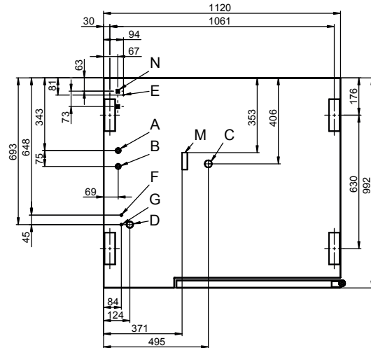
Connection points
